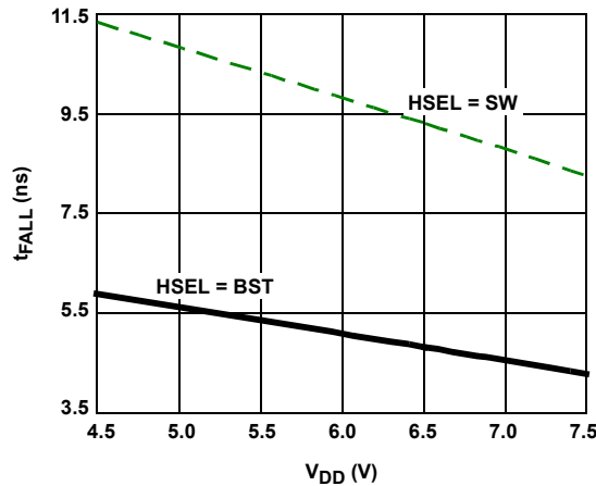
FIGURE 24. HIGH-SIDE DRIVER FALL TIME, t_{FH} (CGH = 3nF, T_A = +25°C)
