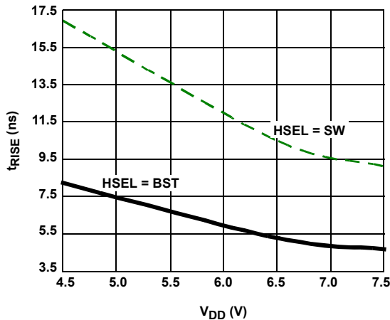
FIGURE 22. HIGH-SIDE DRIVER RISE TIME, t_{RH} (CGH = 3nF, T_A = +25°C)
