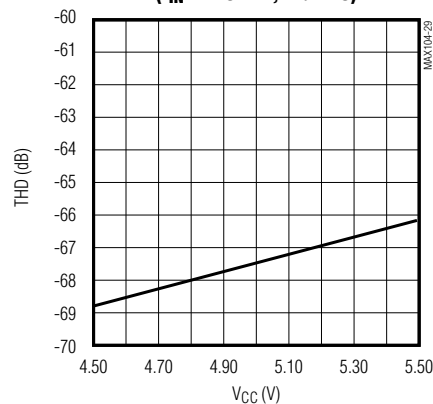
TOTAL HARMONIC DISTORTION vs. V_{CCI} = V_{CCA} = V_{CCD} ( f_{IN} = 125MHz , -1dB FS)
