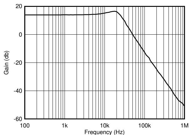
Figure 7-2. OPA132 2nd-Order 30kHz, Low-Pass Filter Response
