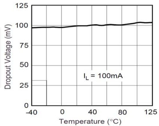
Figure 20. Dropout Voltage
