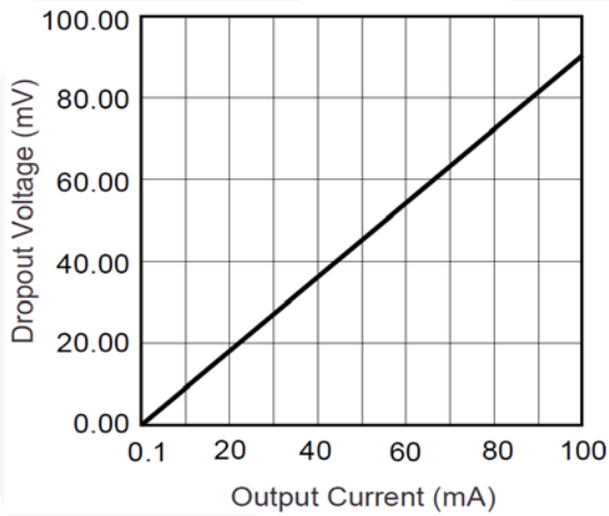
Figure 17. Dropout Voltage
