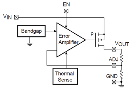
Figure 1. Block Diagram
