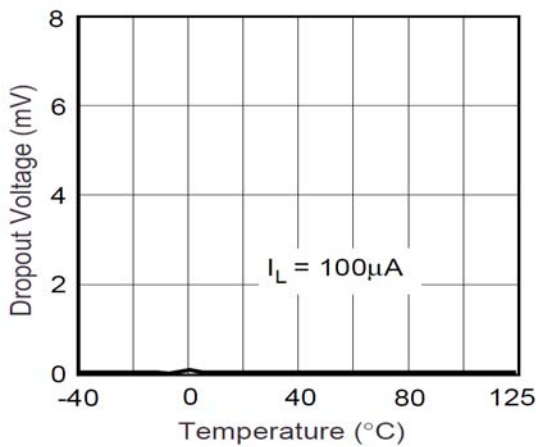
Figure 19. Dropout Voltage
