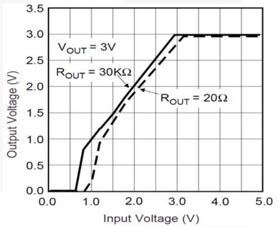
Figure 18. Dropout Characteristics
