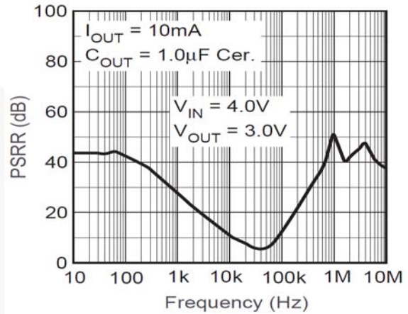
Figure 4. Power Supply Rejection Ratio
