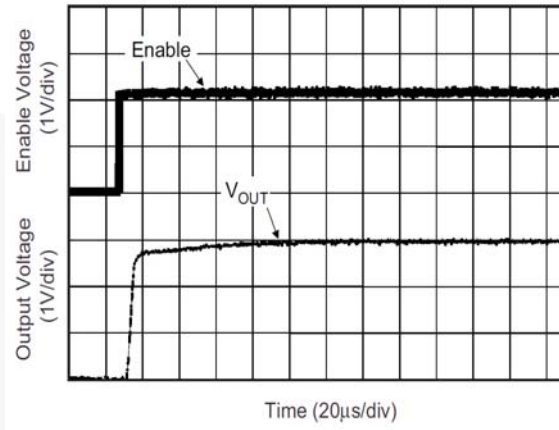
Figure 22. Enable Pin Delay
