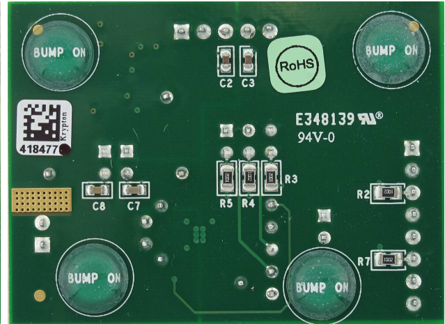
Figure 3. SN65HVD01-EVM Bottom View
