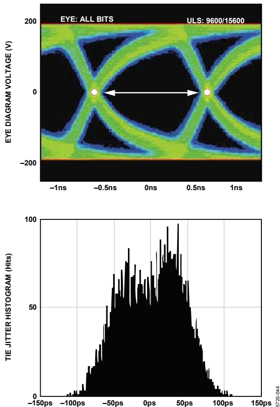
Figure 62. Data Eye for LVDS Outputs in ANSI-644 Mode with Trace Lengths Greater than 24 Inches on Standard FR-4, External 100 \Omega Far Termination Only
