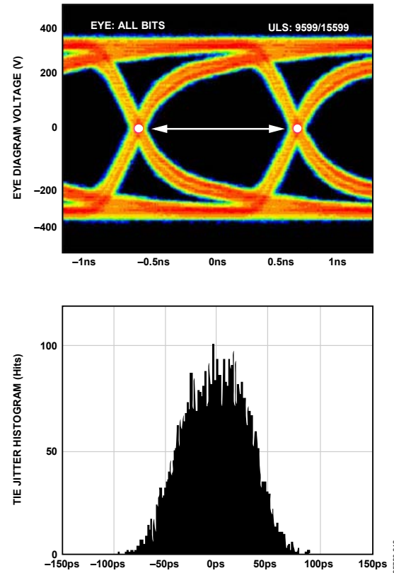
Figure 63. Data Eye for LVDS Outputs in ANSI-644 Mode with 100 \Omega Internal Termination on and Trace Lengths Greater than 24 Inches on Standard FR-4, External 100 \Omega Far Termination Only
