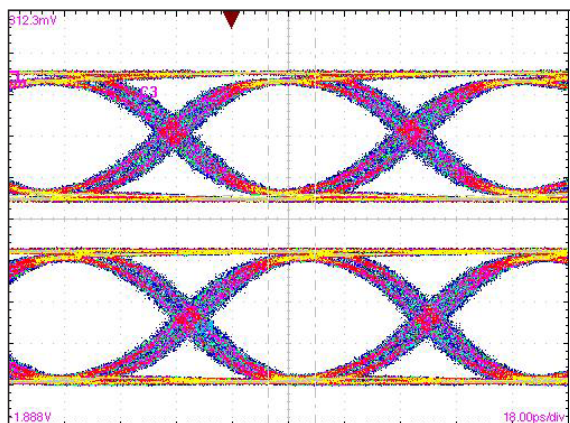
Eye Diagram
