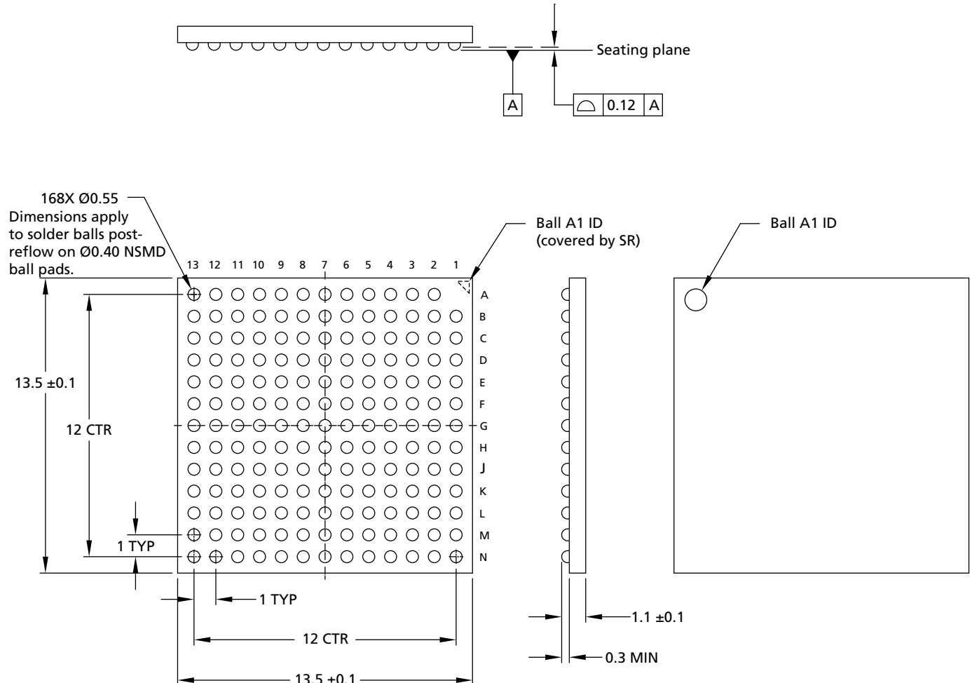
Figure 5: 168-Ball FBGA
