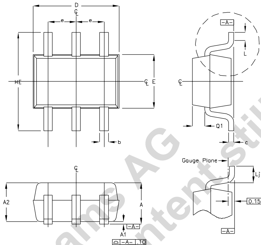
Figure 20. SC70-6 Package
