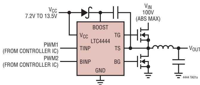
High Input Voltage Buck Converter
