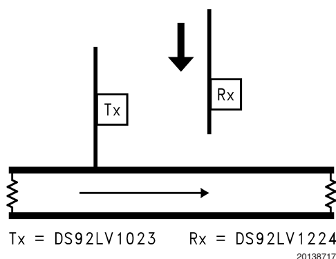
FIGURE 13. Random Lock Hot Insertion
