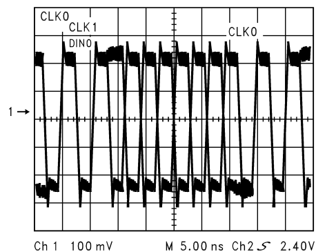
DIN0 Held Low-DIN1 Held High Creates an RMT Pattern
