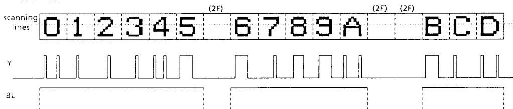
Figure 3-7. Example of Y and BL signal output
