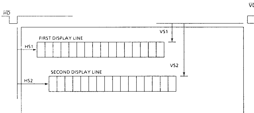
Figure 3-6. TV screen image
