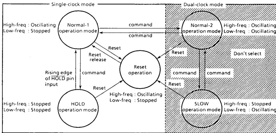
Figure 2-3. Operation Mode Transition Diagram
