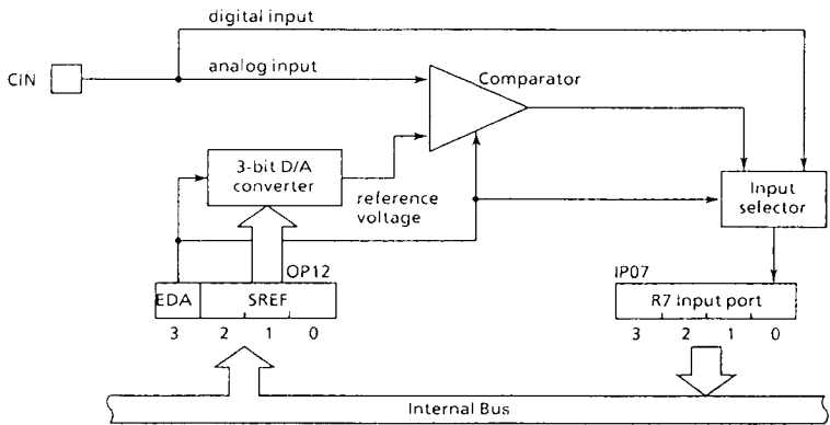
Figure 3-10. Comparator input circuit
