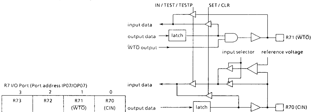
Figure 3-3. Port R7
