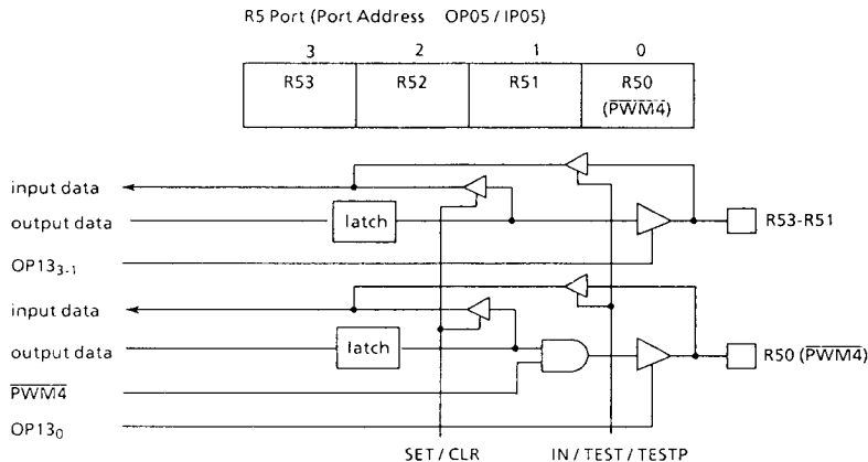
Figure 3-2. Port R5
