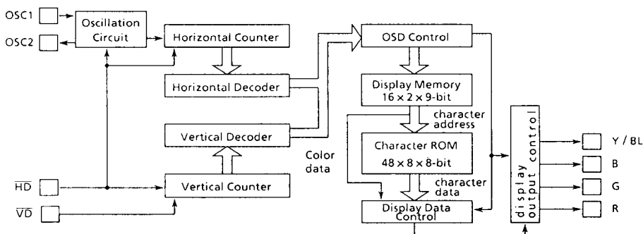
Figure 3-4. OSD Circuit
