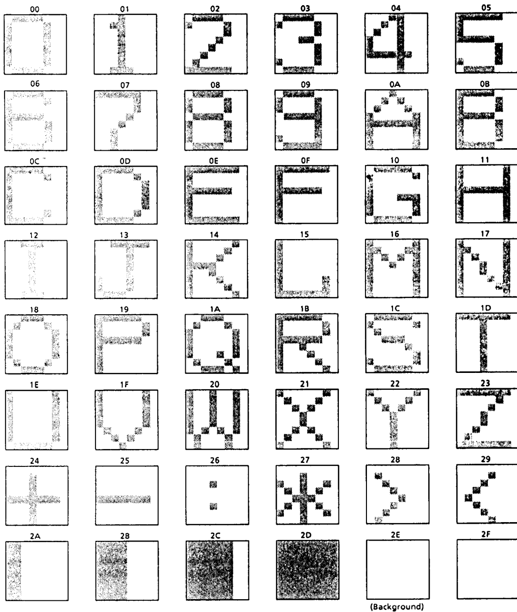
Figure 3-9. Character ROM address and character pattern
