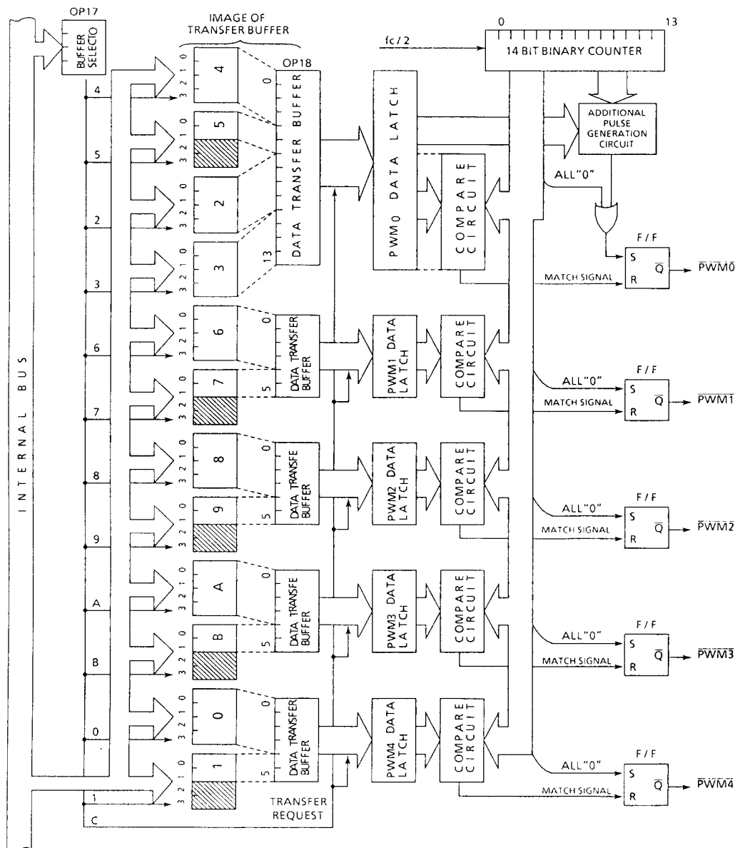
Figure 3-13. Pulse Width Modulation Circuit
