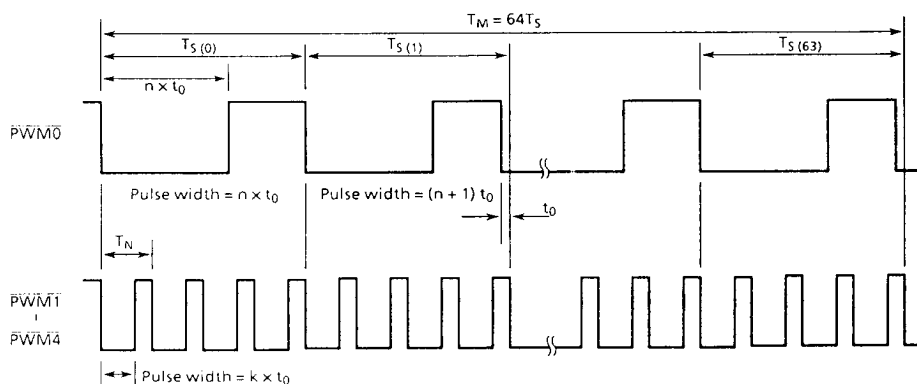
Figure 3-12. \overline{\text{PWM}} Output Waveform (It is shown to the additional pulse T_S(1) and T_S(63) of the \overline{\text{PWM0}} )
