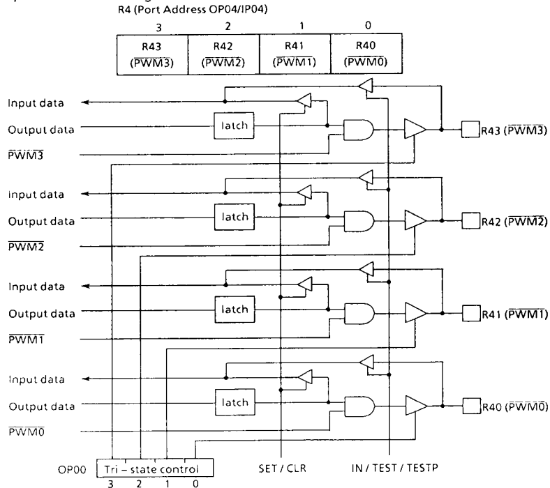
Figure 3-1. Port R4 ( \overline{\text{PWM}} )
