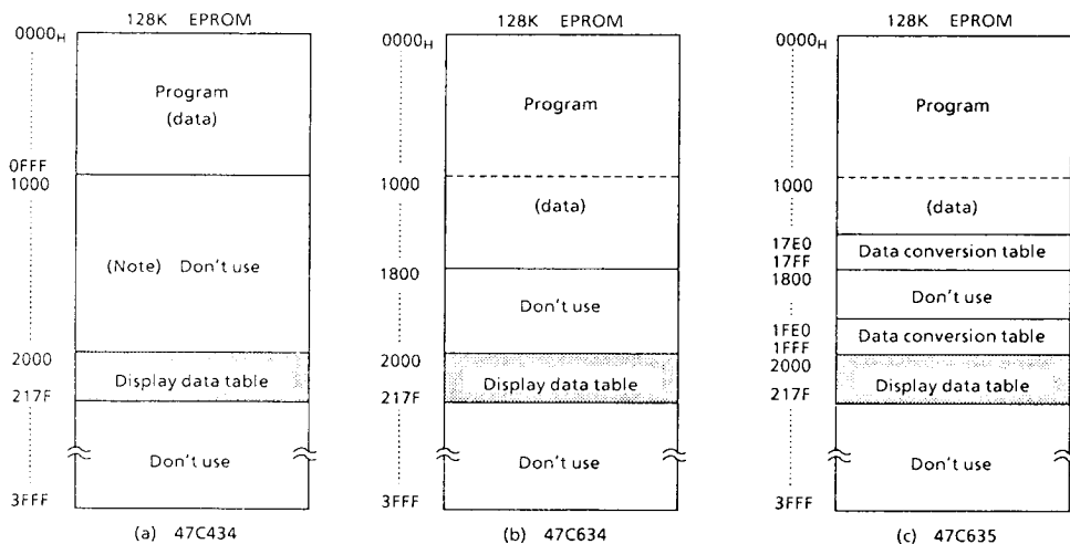
Figure 1. Program area
