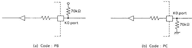
Figure 4. I/O code and external circuitry
