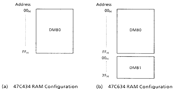
Figure 2-2. Data Memory (RAM)
