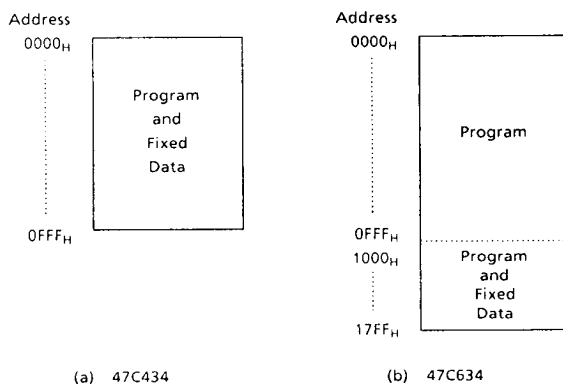
Figure 2-1. Program Memory
