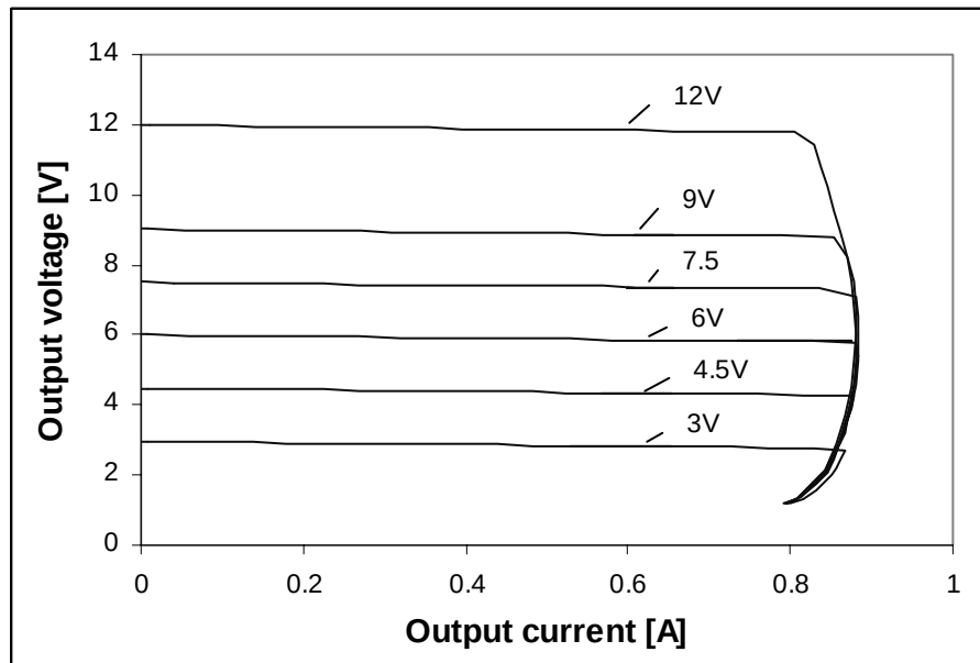
Figure 1 Output Characteristic: U_1 = 230V ; f_1 = 50 \text{ Hz} ; resistive load
