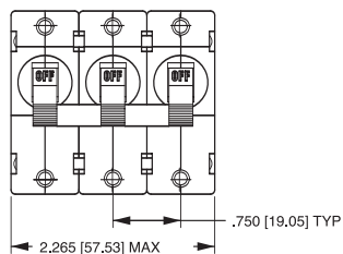
3-POLE (AA3)
