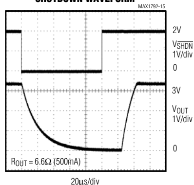
SHUTDOWN WAVEFORM
