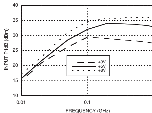
Low Frequency Input P1dB vs. Vctl
