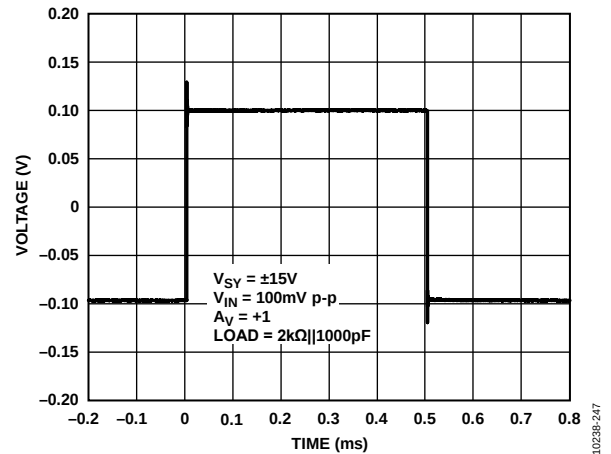
Figure 50. Small Signal Transient Response, V_{SV} = \pm 15\text{ V}
