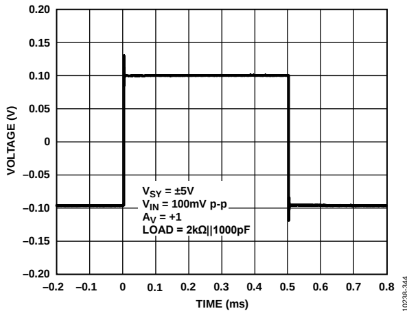
Figure 47. Small Signal Transient Response, V_{SV} = \pm 5\text{ V}
