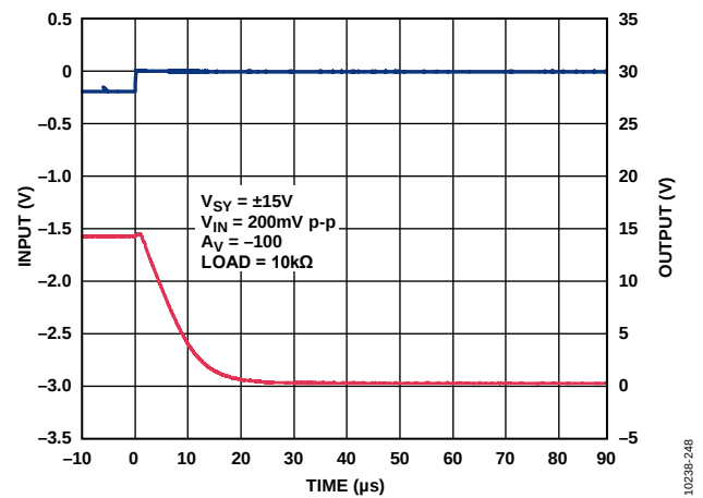
Figure 51. Positive Overload Recovery, V_{SV} = \pm 15\text{ V}
