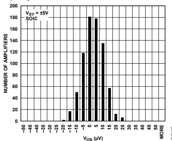
Figure 4. Offset Voltage Distribution
