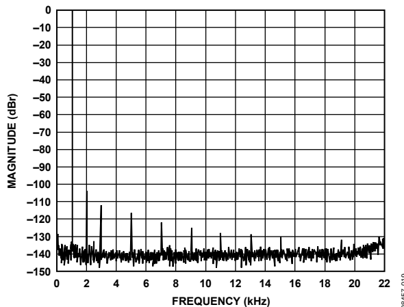
Figure 19. Input 0 dBFS @ 1 kHz, BW 10 Hz to 22 kHz, SR 48 kHz
