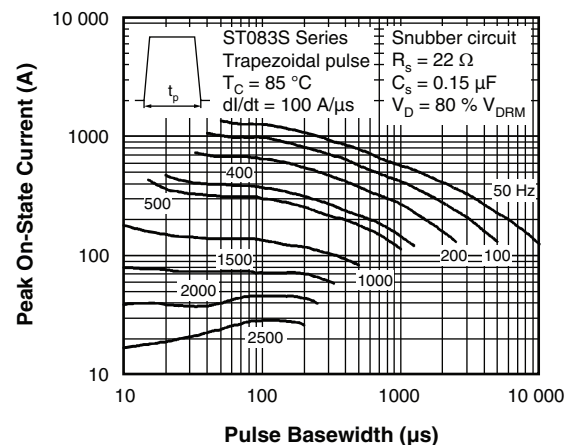
Fig. 13 - Frequency Characteristics
