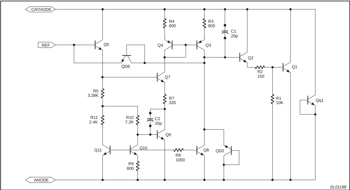
Figure 2. Equivalent Schematic
