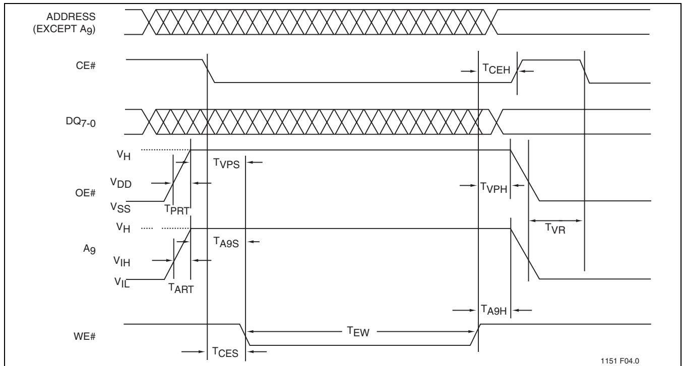
FIGURE 6: Chip-Erase Timing Diagram
