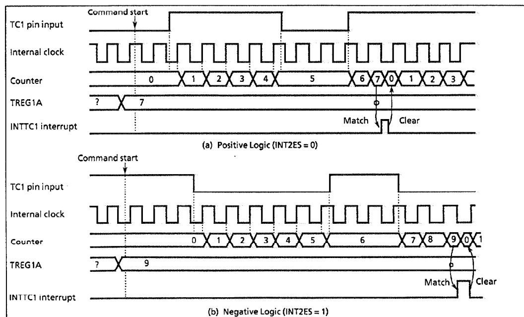
Figure 2-15. Window mode timing chart
