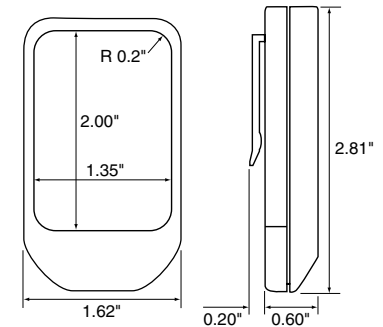
Figure 1: Package Dimensions
