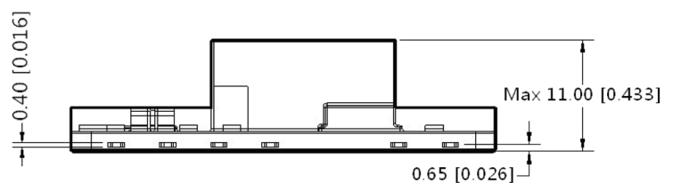
Bottom View
