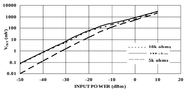
Detector Output Voltage vs Input Power and Load Resistance. Diode at Zero Bias. Untuned Fixture at 9.375 GHz
