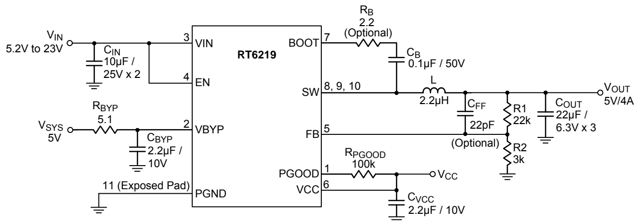
Figure 1. Typical Application Circuit for V_{OUT} = 5V
