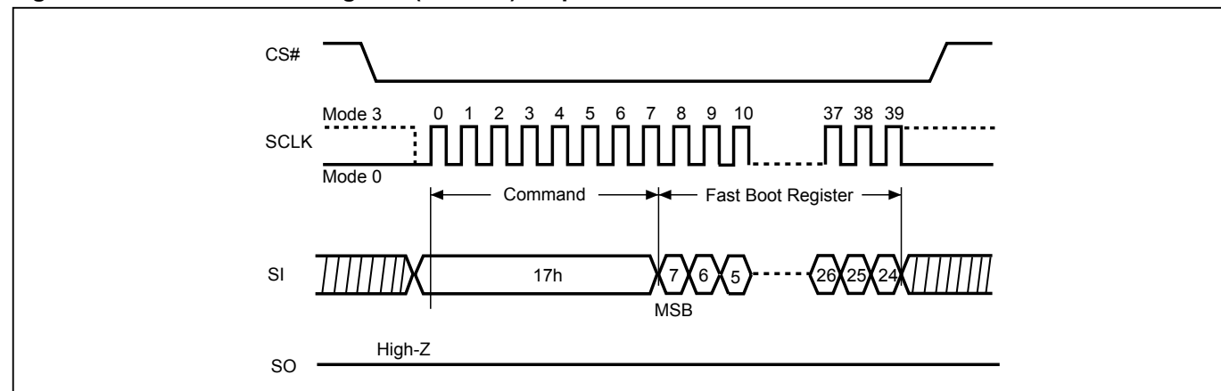
Figure 41. Write Fast Boot Register (WRFBR) Sequence
