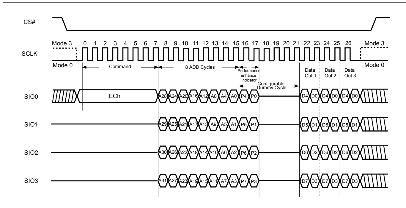
Figure 33. 4 I/O Fast Read using 4 Byte Address sequence (4READ4B)
