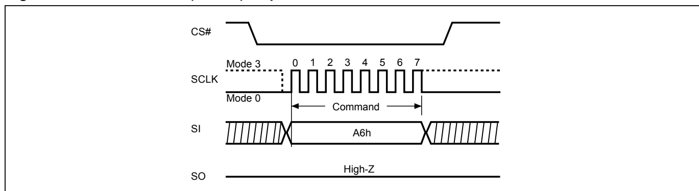
Figure 60. SPB Lock Bit Set (SPBLK) Sequence
