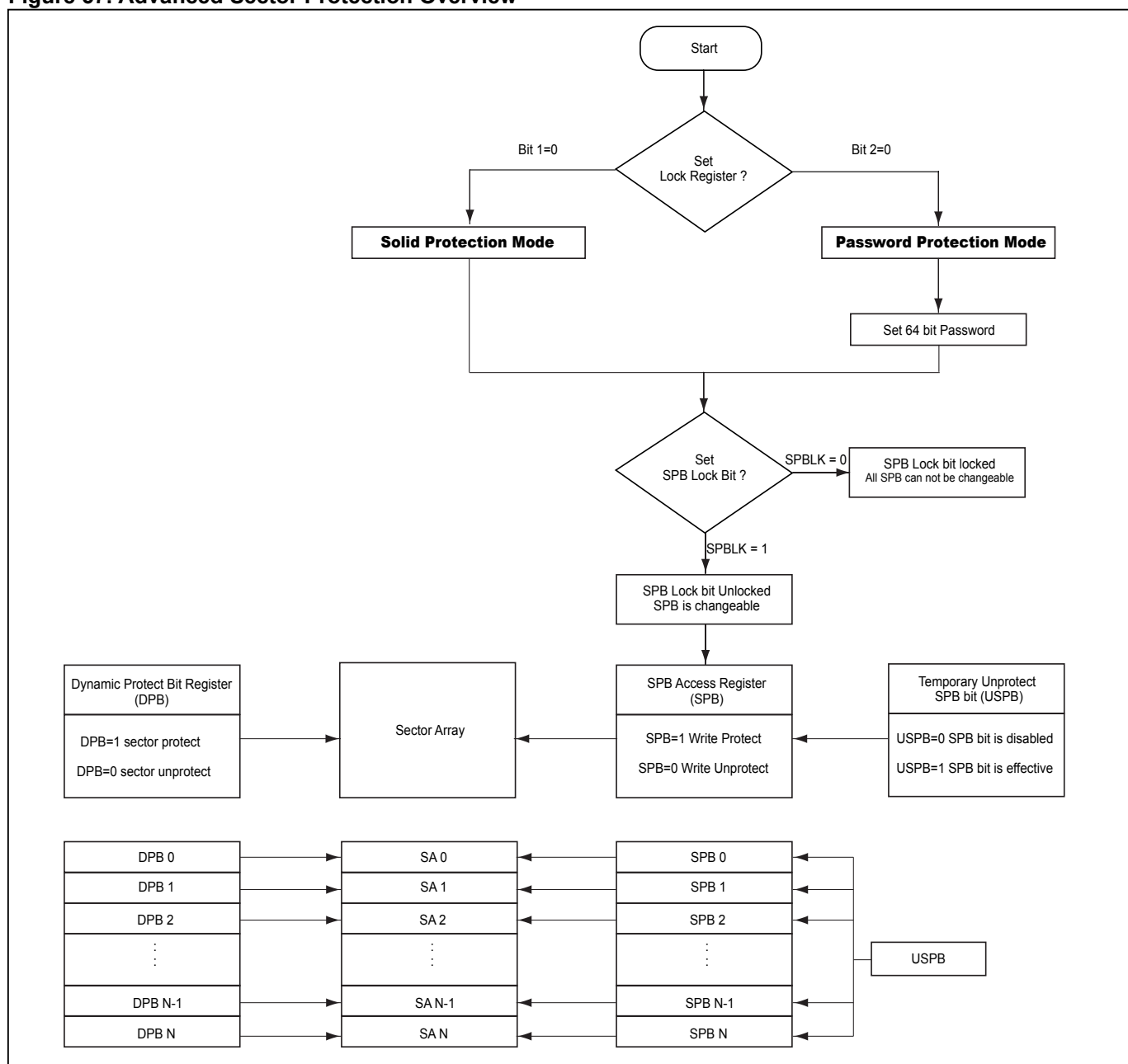
Figure 57. Advanced Sector Protection Overview
