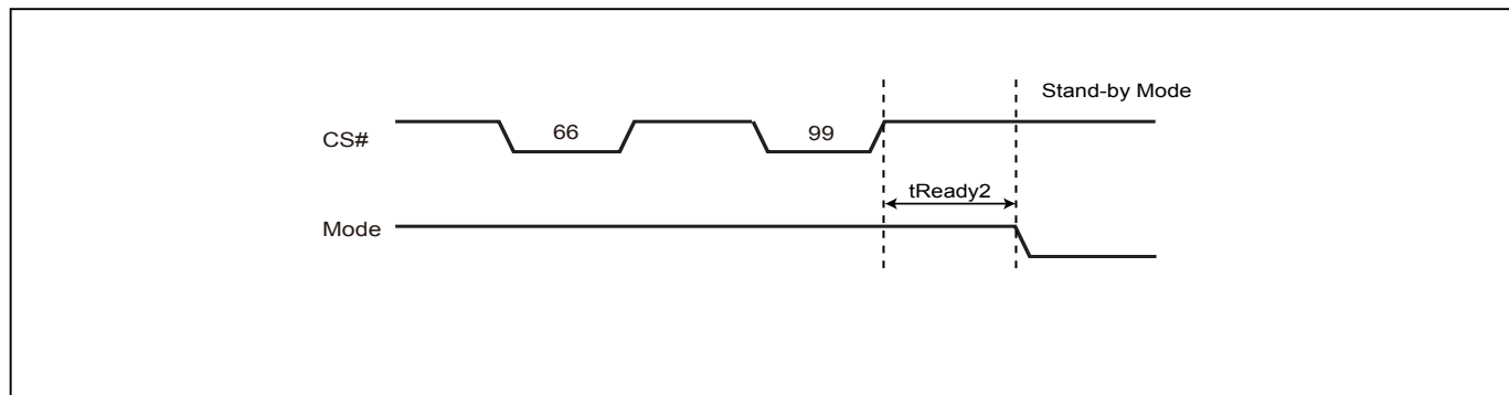
Figure 70. Software Reset Recovery
