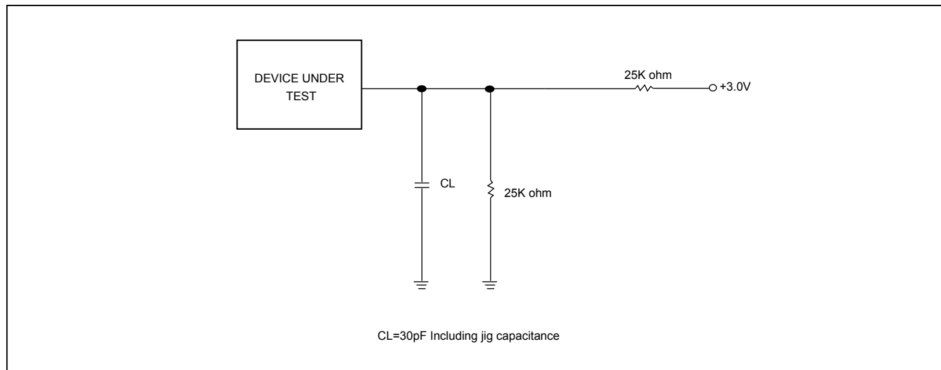
Figure 78. OUTPUT LOADING
