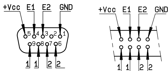
D-Sub connector
