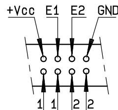
Solder pins
