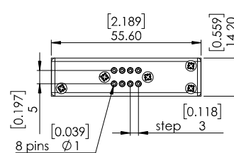
TOP view - solder pins
