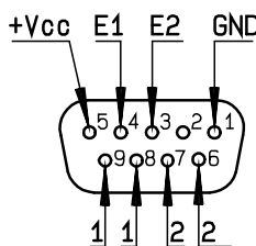
D-Sub connector
