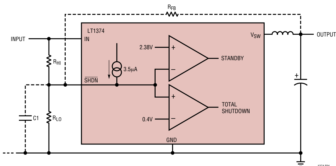
Figure 4. Undervoltage Lockout
