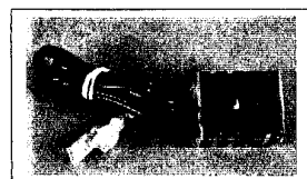
Part No. 917D9. Voltage Regulator. (6-15v DC Input, 3v, 1.5amp output) Part No. 917D10. Voltage Regulator. (6-15v DC Input, 1.5v, 1.5amp output) Part No. 917D11. Voltage Regulator. (6-15v DC Input, 4.5v, 1.5amp output) (Above for 280 motor only)
