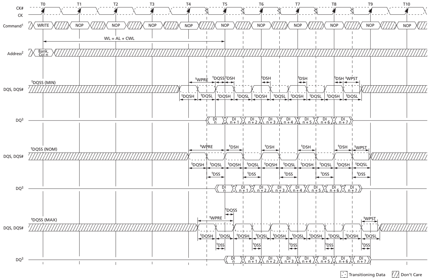
Figure 83: WRITE Burst
