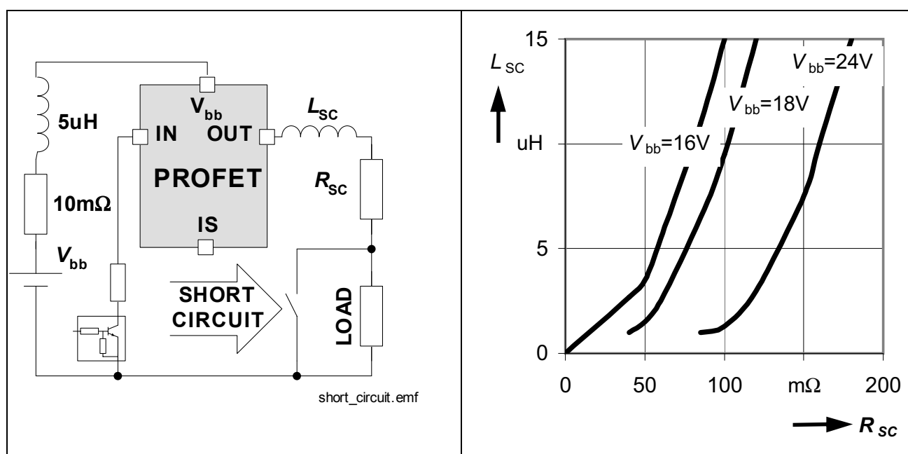
Figure 13 Short circuit
