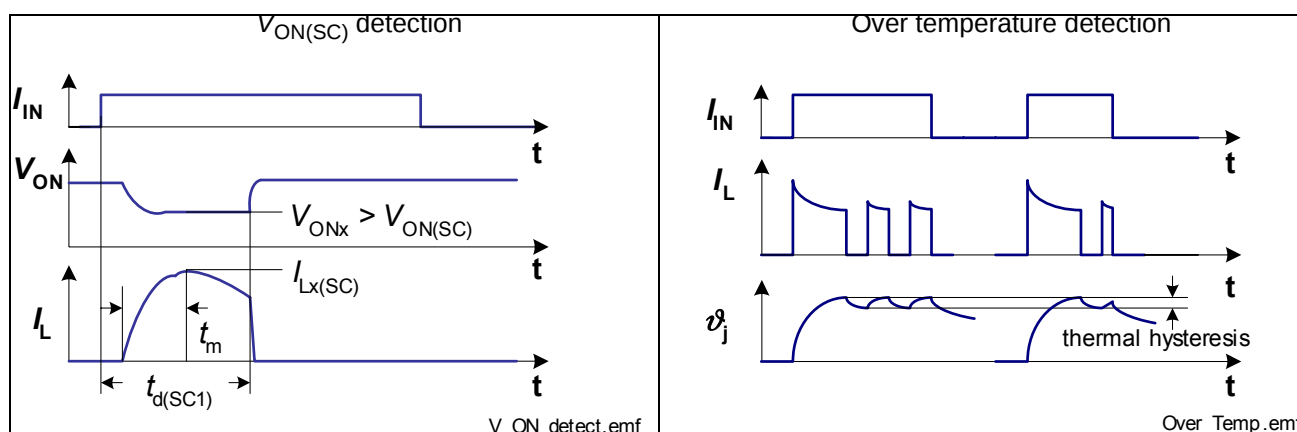
Figure 12 Overload Behavior
