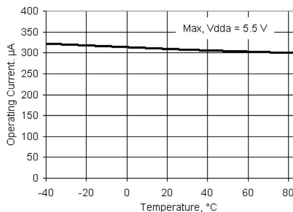
Figure 11-57. VDAC Operating Current vs Temperature, 1 V Mode, Fast Mode
