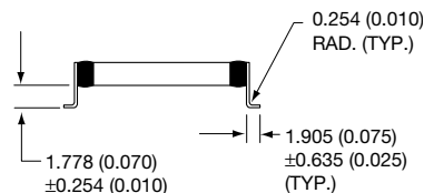
"L" STYLE LEADS
