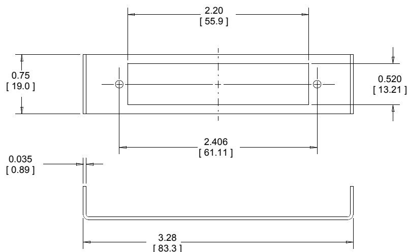
Latch Bracket
