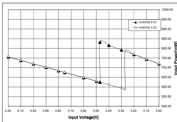
Input Power of SC600 B&D Output Current = 120mA
