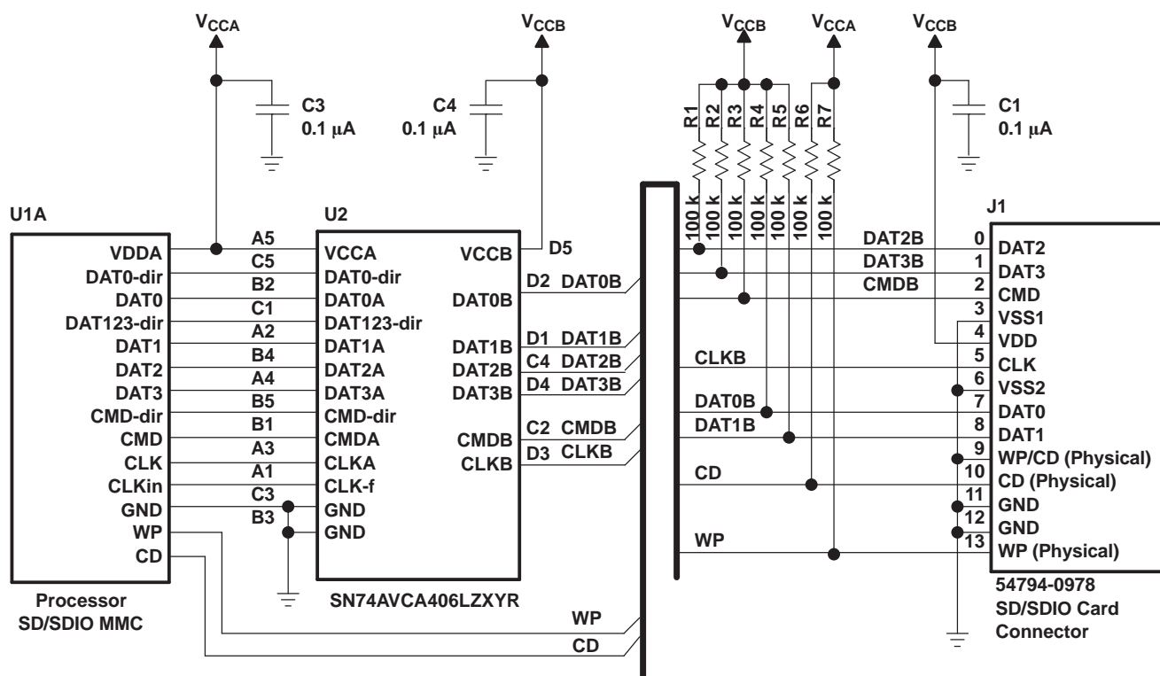
Figure 1. Interfacing With SD/SDIO Card
