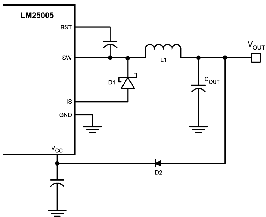
FIGURE 12. VCC Bias from VOUT for 8V &lt; VOUT &lt; 14V
