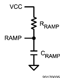
FIGURE 7. R_{RAMP} to V_{CC} for V_{OUT} > 7.5V
