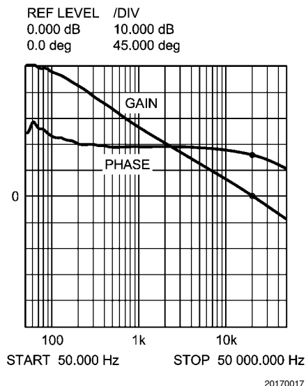
FIGURE 11. Overall Loop Gain and Phase
