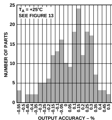
Figure 12. Output Accuracy Distribution, V_{OUT} = 2.8 V
