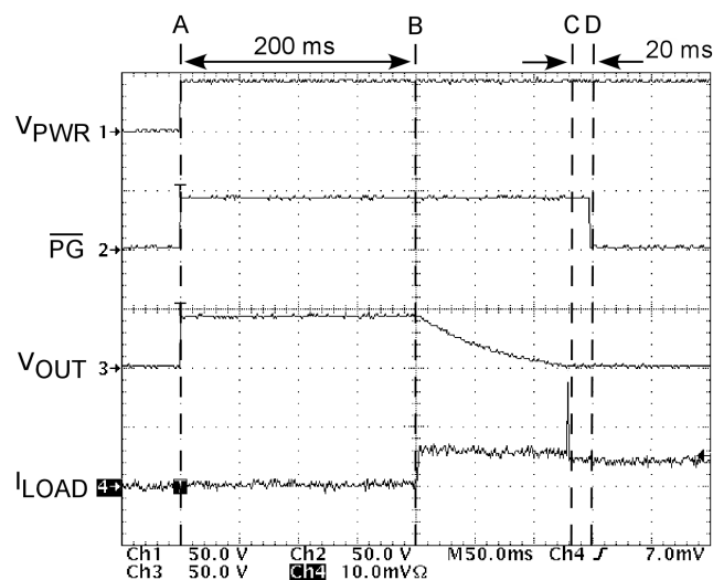
Figure 6. Start-Up Sequence
