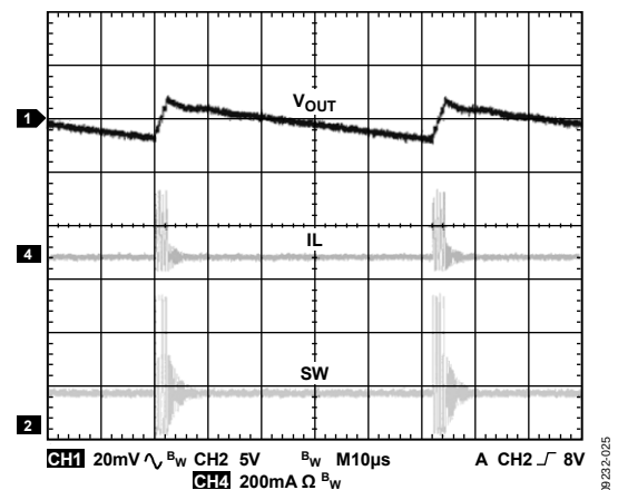
Figure 7. Steady State at Light Load, f_{SW} = 1.4\text{ MHz} , I_{OUT} = 40\text{ mA}
