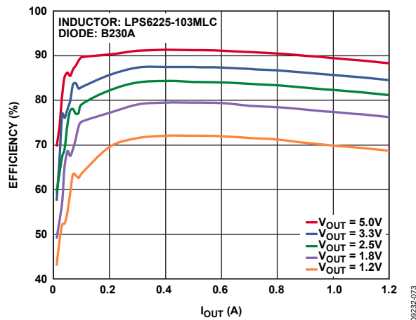
Figure 3. Efficiency Curve, V_{IN} = 12\text{ V} , f_{SW} = 700\text{ kHz}
