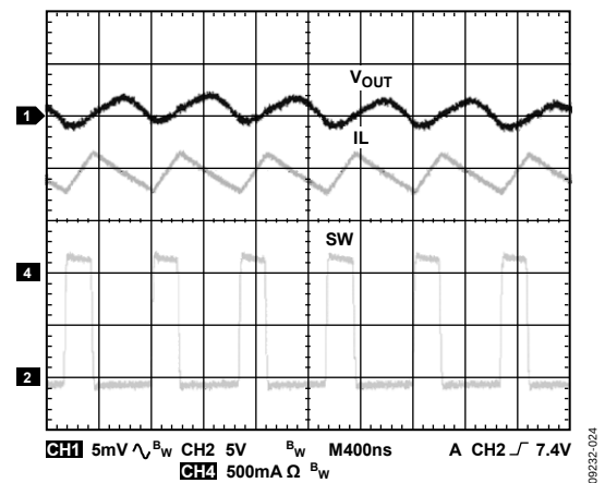
Figure 6. Steady State at Heavy Load, f_{SW} = 1.4\text{ MHz} , I_{OUT} = 1\text{ A}
