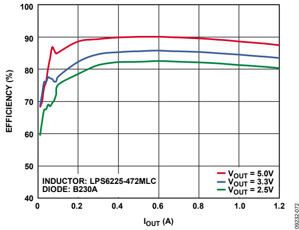
Figure 2. Efficiency Curve, V_{IN} = 12\text{ V} , f_{SW} = 1.4\text{ MHz}
