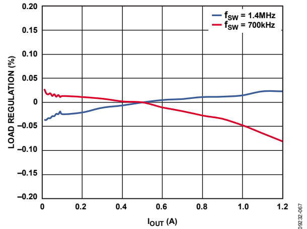
Figure 5. Load Regulation, V_{OUT} = 3.3\text{ V} , V_{IN} = 12\text{ V}
