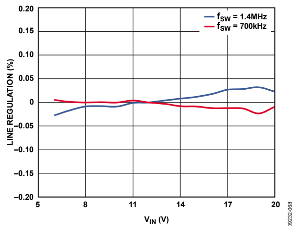
Figure 4. Line Regulation, V_{OUT} = 3.3\text{ V} , I_{OUT} = 500\text{ mA}
