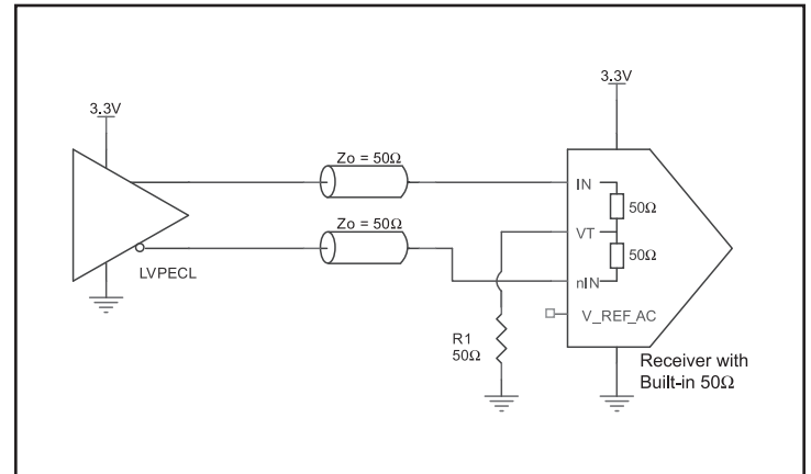
Figure 2B. IN/nIN Input with Built-In 50 \Omega Driven by an LVPECL Driver
