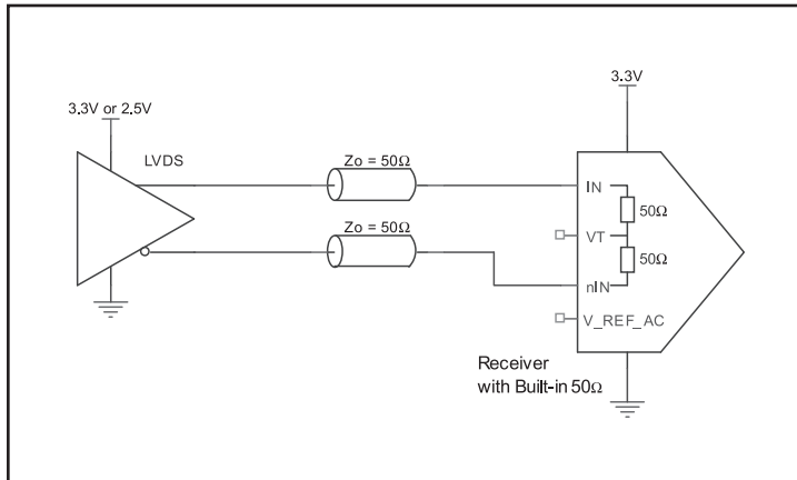
Figure 2A. IN/nIN Input with Built-In 50 \Omega Driven by an LVDS Driver
