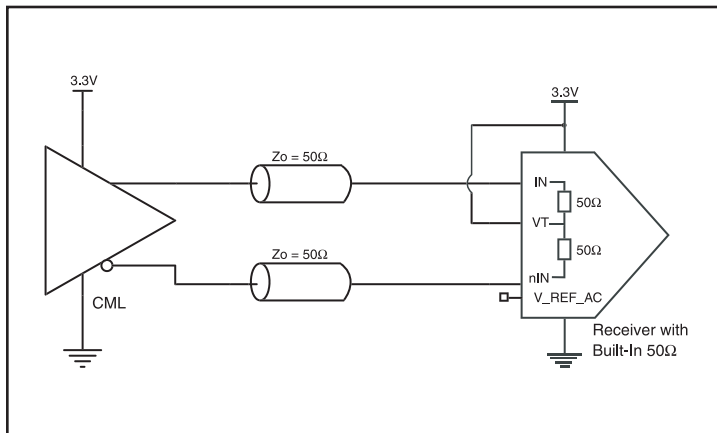
Figure 2C. IN/nIN Input with Built-In 50 \Omega Driven by a CML Driver
