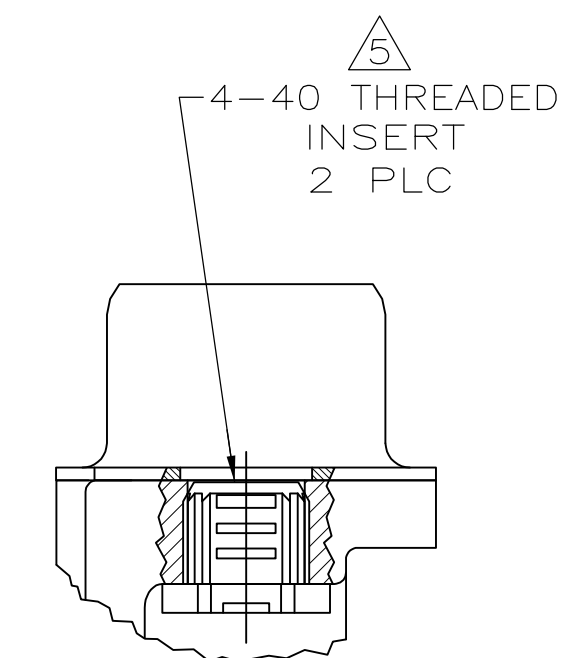
DETAIL D
