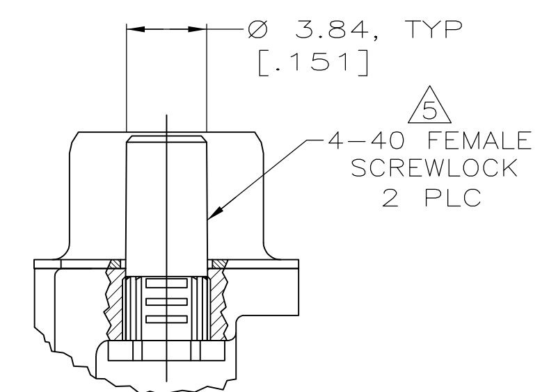
DETAIL E
