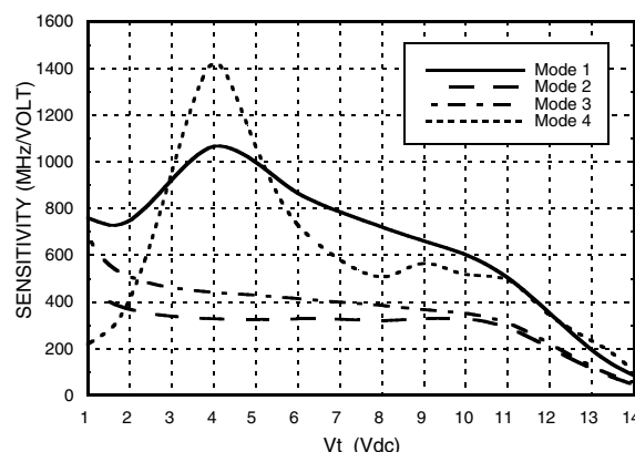
Tuning Sensitivity Vs. V_t
