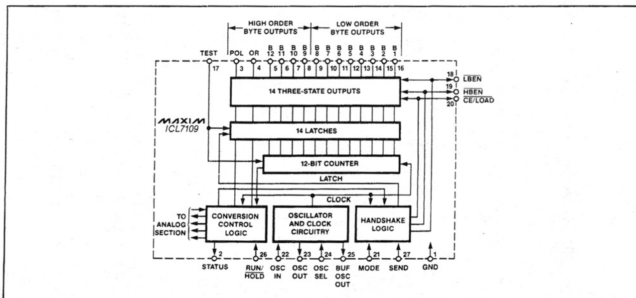
Figure 4. Digital Section
