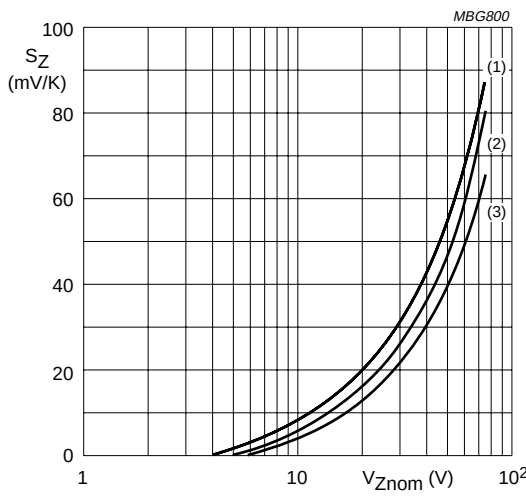
I_Z = I_{Ztest} ; T_j = 25 \text{ to } 150 \text{ }^\circ C . (1) Maximum values. (2) Typical values. (3) Minimum values.
