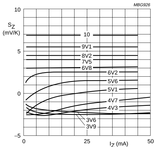
BZV85-C3V6 to C10. T_j = 25 \text{ to } 150 \text{ }^\circ C . For types above 7.5 V the temperature coefficient is independent of current; see Table "Per type".
