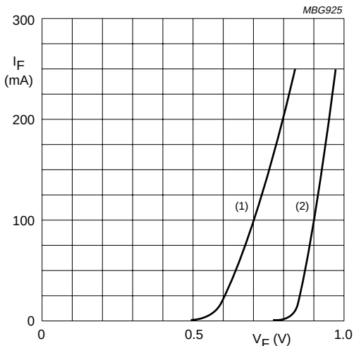
(1) T_j = 200 \text{ }^\circ C . (2) T_j = 25 \text{ }^\circ C .
