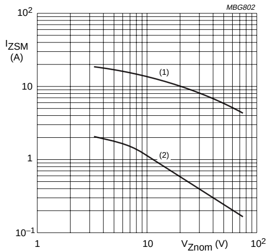
(1) t_p = 10 \mu s ; half sinewave; T_{amb} = 25 \text{ }^\circ C . (2) t_p = 10 ms ; half sinewave; T_{amb} = 25 \text{ }^\circ C .
