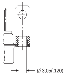
Plastic Bracket with Bushing (1A5N)
