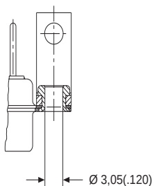
Metal Bracket with Bushing (1AFN)
