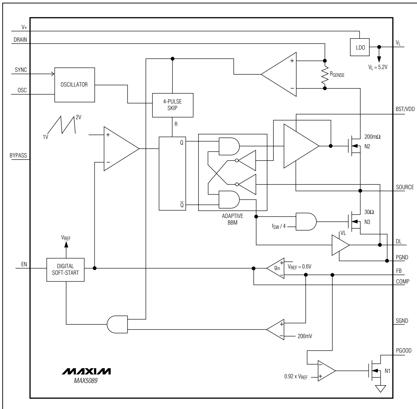
Figure 2. MAX5089 Block Diagram
