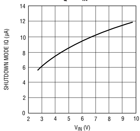
Shutdown I_{\text{Q}} vs V_{\text{IN}}
