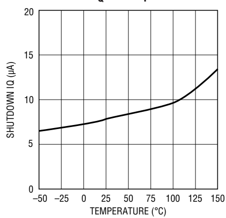
Shutdown I_{\text{Q}} vs Temperature
