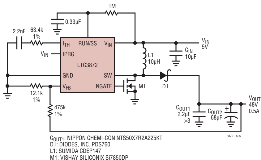
Soft-Start
