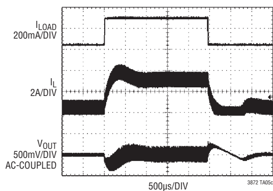
Load Step
