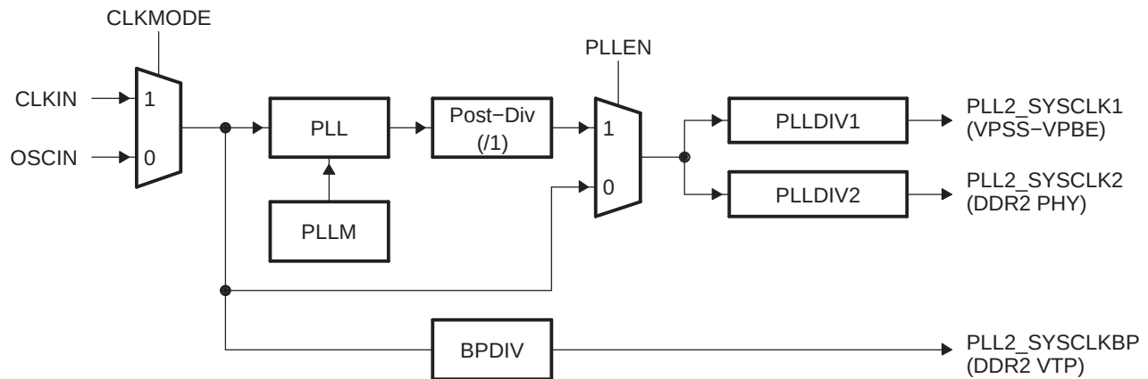
Figure 5-8. PLL2 Structure Block Diagram
