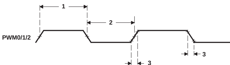
Figure 5-70. PWM Output Timing
