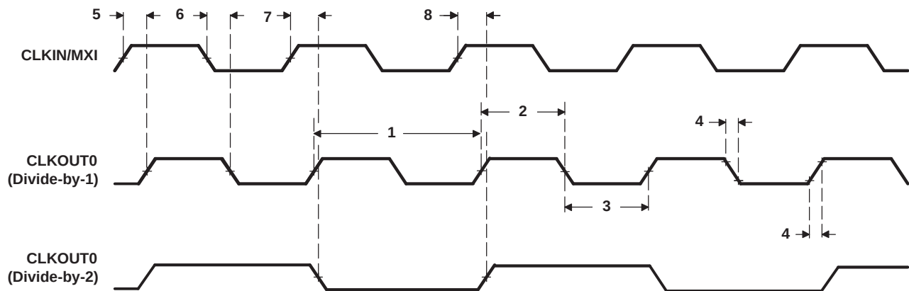
Figure 5-14. CLK_OUT0 Timing
