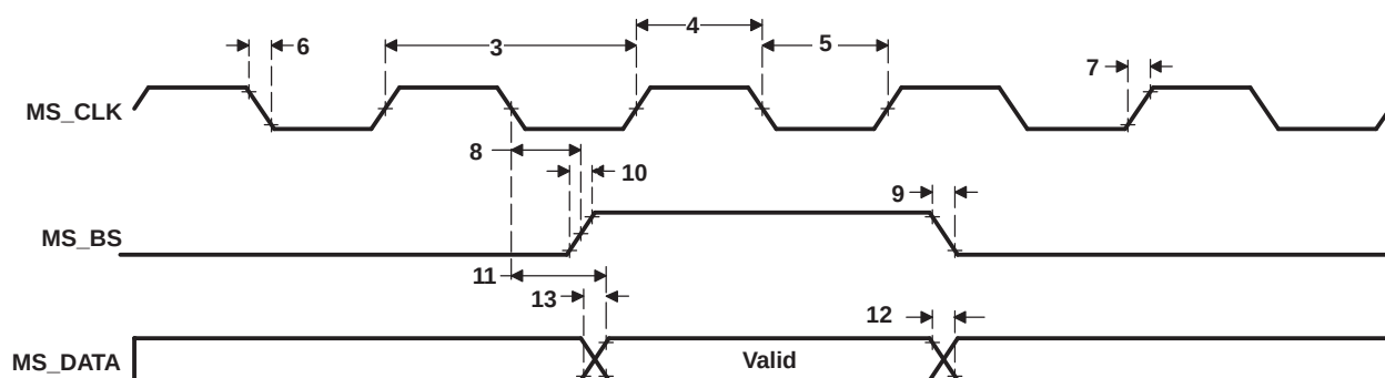
Figure 5-75. MS/MS PRO Serial Interface Output Timing
