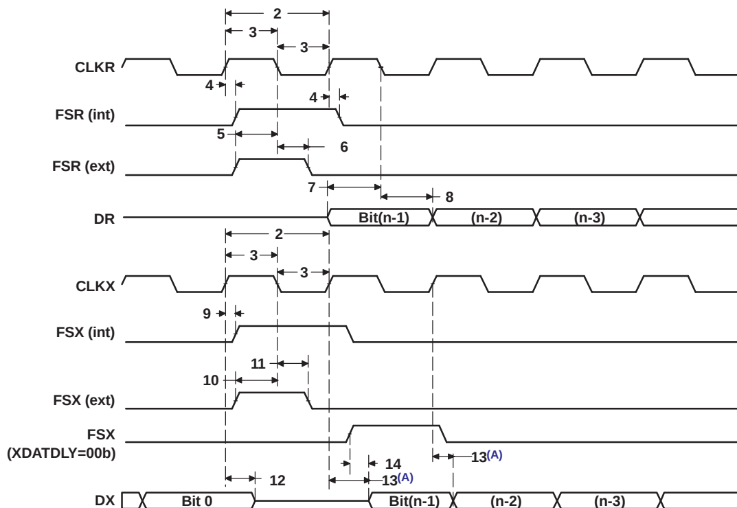
Figure 5-62. ASP Timing
