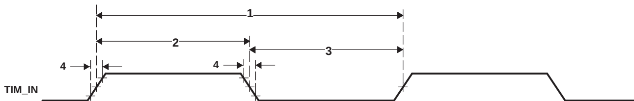
Figure 5-69. Timer Timing
