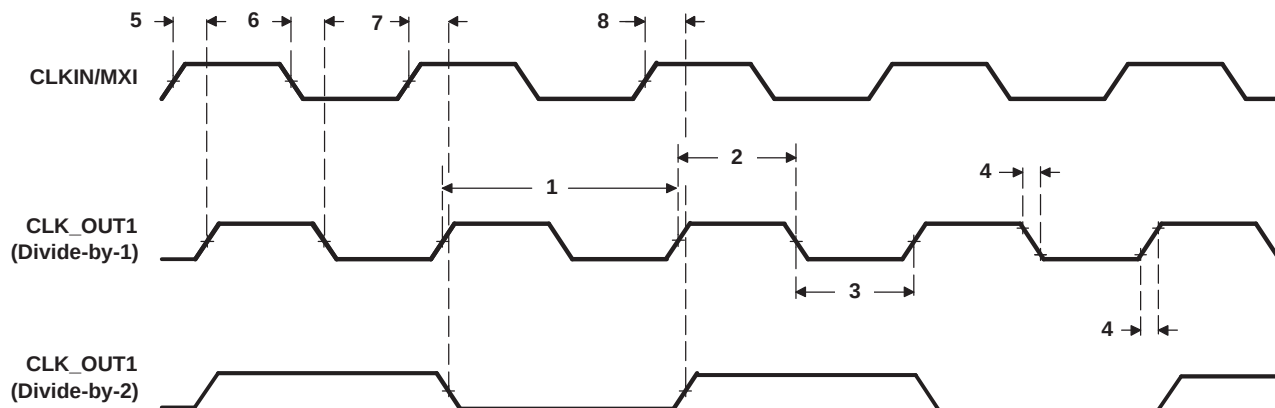
Figure 5-15. CLK_OUT1 Timing
