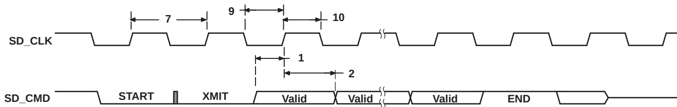
Figure 5-41. MMC/SD/SDIO Card Response Timing
