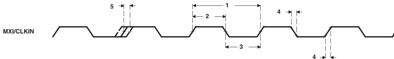
Figure 5-13. M24XI Timing
