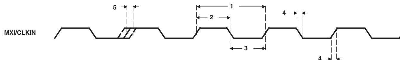
Figure 5-12. MXI/CLKIN Timing
